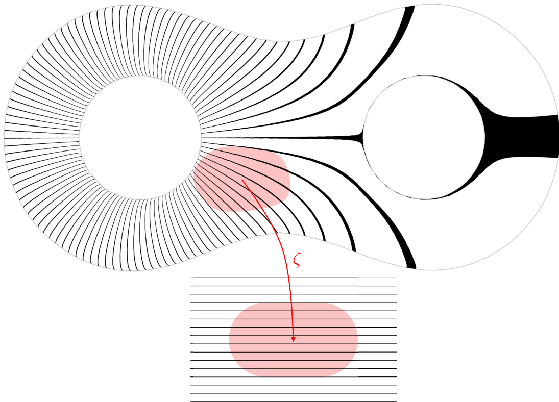
FIGURE 2.2: Natural coordinates map the leaves of the vertical foliation of a holomorphic quadratic differential to horizontal lines in the plane.
